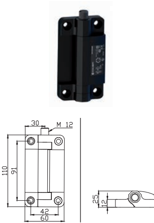
Top axial exit with M12 connector
