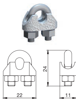
Rope Clamp
