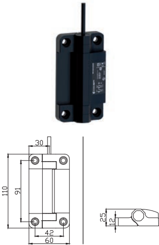
Top axial exit with cable
