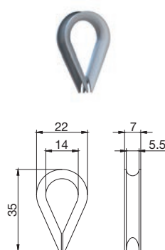
Rope eye
