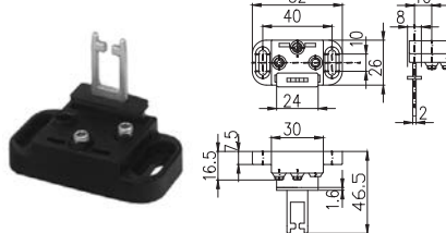
Order code 49: Adjustable joint key
