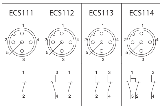
M12 Connector 5 poles
