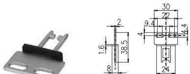
Order code 4: Flat key
