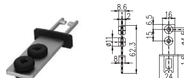
Order code 8: Shock absorbing flat key
