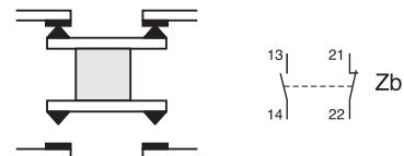
The 2 moving contacts are electrically separated
