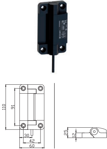
Bottom axial exit with cable
