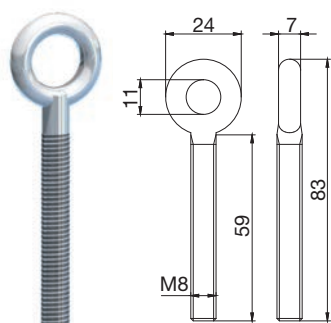
Stay Bolt
